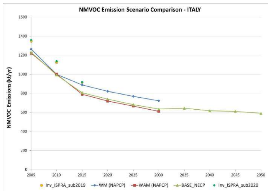
Figure 9.18 –Reported and projected (WM, WAM, BASE_NECP) NMVOC emissions elaborated by the GAINS-Italy model.
